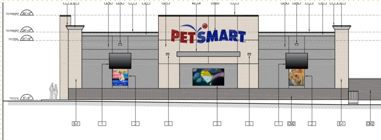
3 WEST ELEVATION 3/32" = 1'-0"
