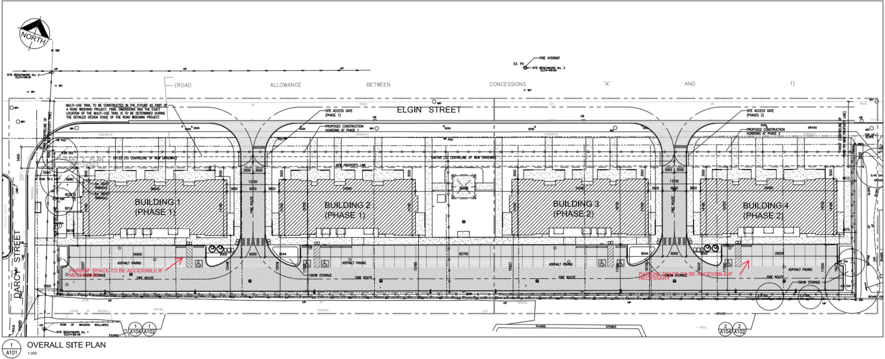
Figure 1 – Overall Site & Phasing Plan
