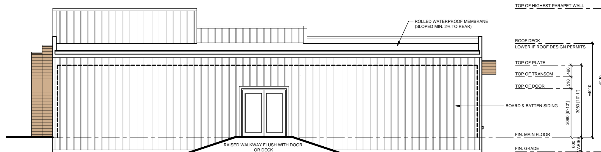
REAR (NORTH) ELEVATION
