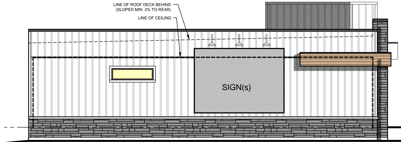
LEFT SIDE (WEST) ELEVATION
