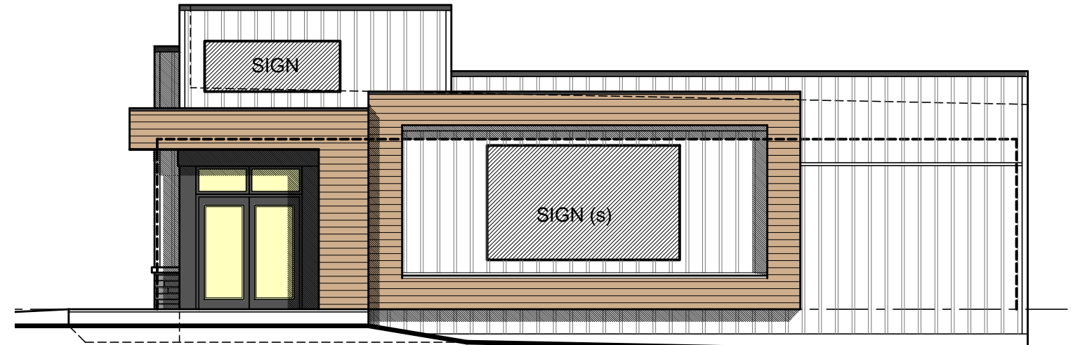
RIGHT SIDE (EAST) ELEVATION FACING PARKING LOT
